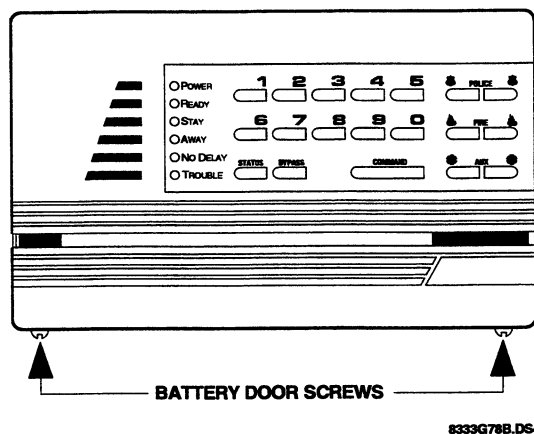
Figure 5. Loosen the two battery door screws
